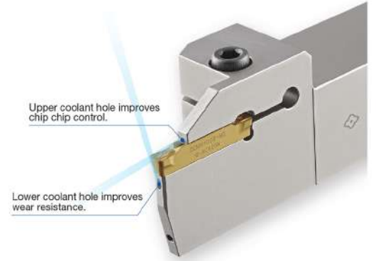
TOOL HOLDERS
